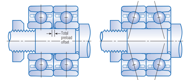
Fig. 8. DB mounting.
