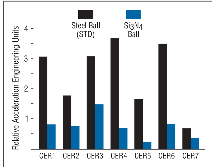
Vibration tests comparing spindles with steel ball bearings and the same spindle retrofit with ceramic hybrids. Vibration levels averaged two to seven times lower with silicon nitride balls.
