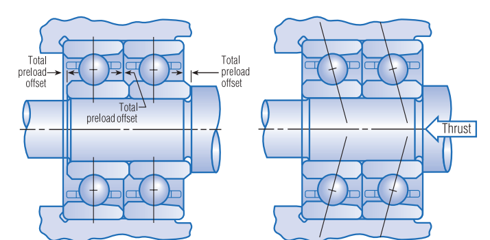
Fig. 10. DT mounting.
