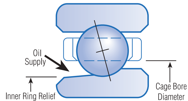
Fig. 17. Lubrication window for B-type bearings.
