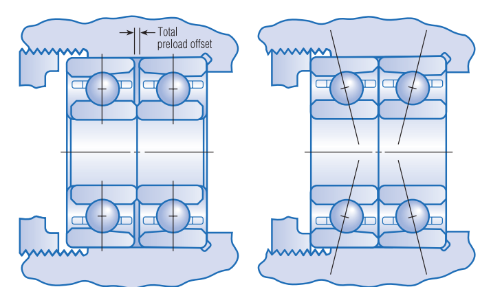
Fig. 9. DF mounting.
