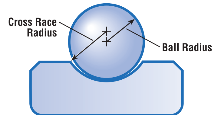
Fig. 2. Raceway curvature.
